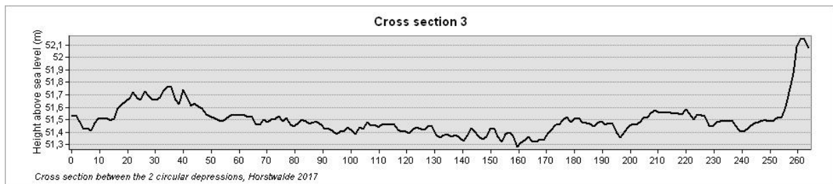
Figure 11: cross section between the 2 depressions, orientated in a North to South direction.
