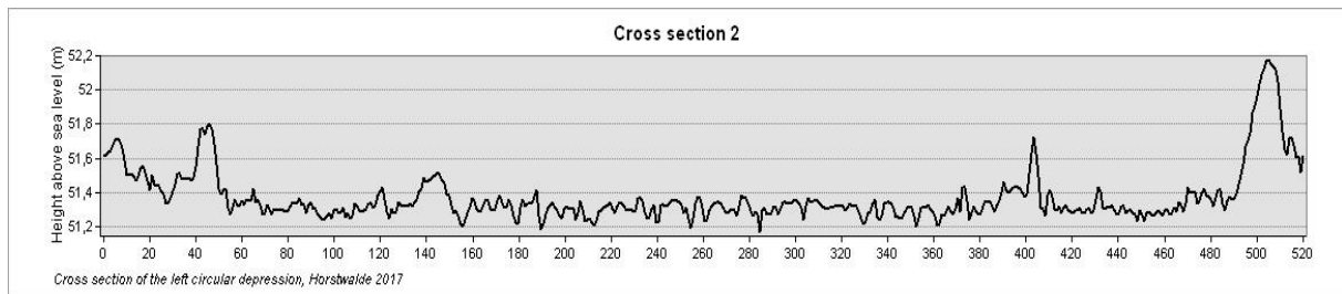
Figure 10: Cross section of depression 1, orientated in a North to South direction.
