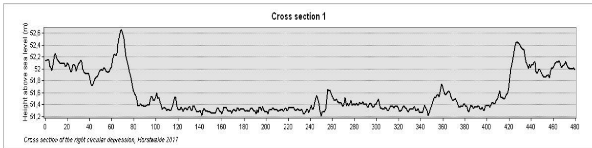
Figure 9: Cross section of depression 2, orientated in a North to South direction.
